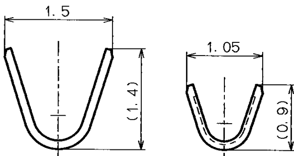
INSULATION BARREL
